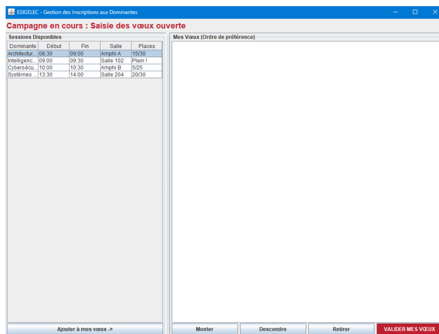
Figure 2 - StudentDashboard
