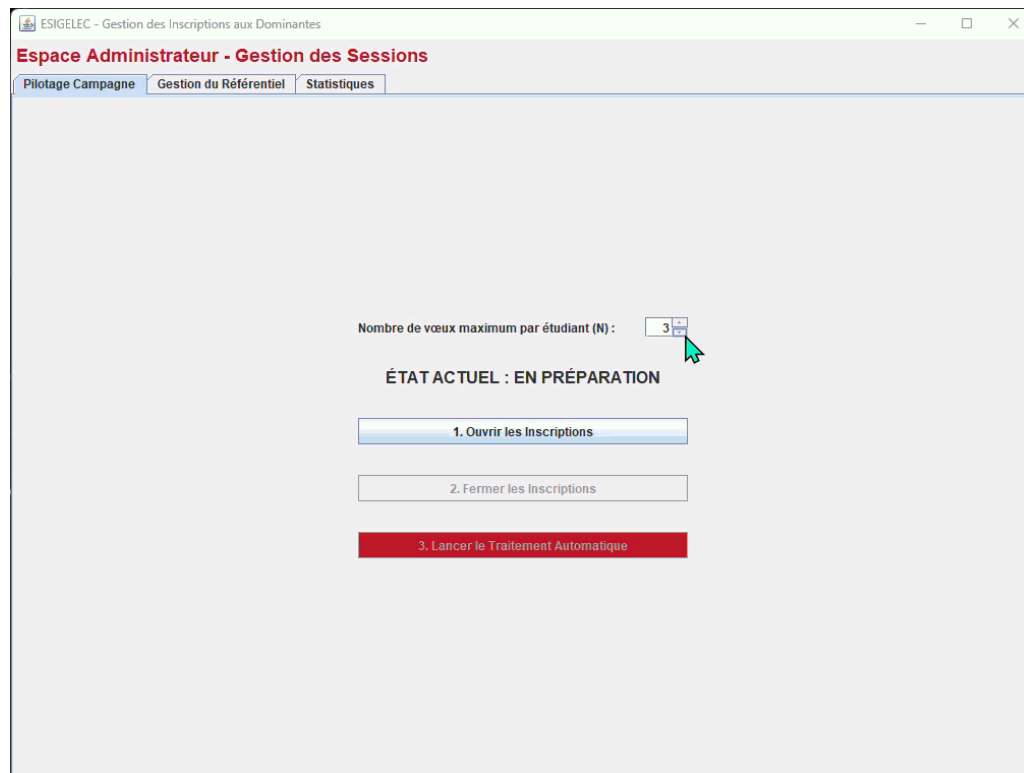
Figure 1 - AdminView
